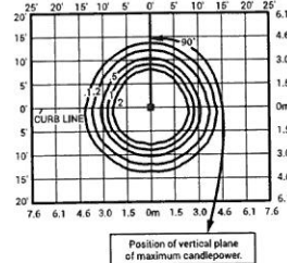
PWY-EDG-5S-**-02-E-UL-350-40K Mounting Height: 3' (0.9m) A.F.G. Initial Delivered Lumens: 1,868 Initial FC at grade
